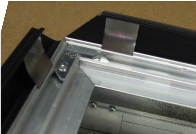
PROFILE OF LIGHTBOX, 4-1/4"D SHOWN DETAIL OF SNAP FRAME
