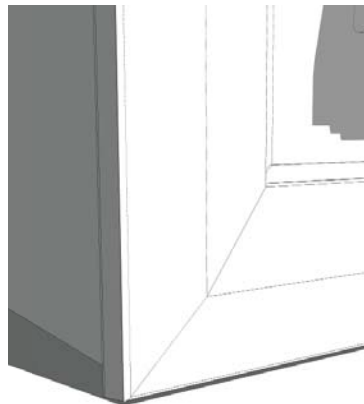
PROFILE OF LIGHTBOX, 4-1/4"D SHOWN DETAIL OF SNAP FRAME
